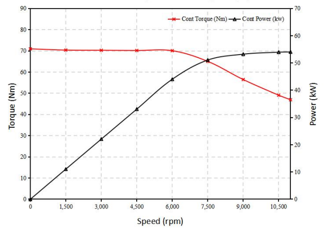
Continuous Torque/Power vs. Speed (S1)
