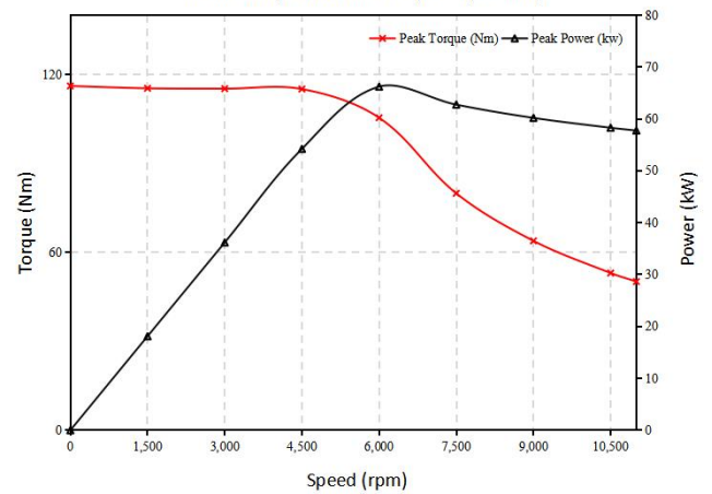
Peak Torque/Power vs. Speed (S2-30s)
